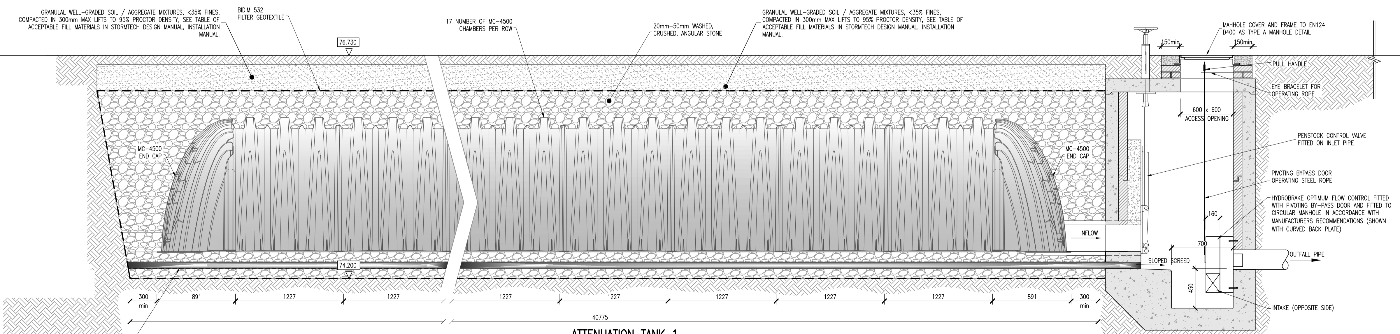
ATTENUATION TANK 1 SECTION B-B THROUGH STORMTECH MC-4500 SCALE 1:25
